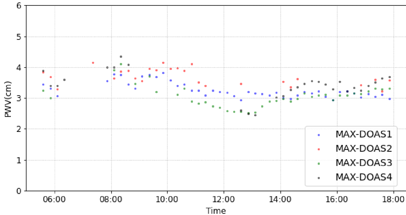
PWV(cm) of MAXDOAS1-4 in Chiba 2021/07/26
